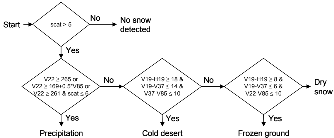
Figure 3-1: SSM/I brightness temperature snow detection algorithm (Ferraro et al., 1996)
