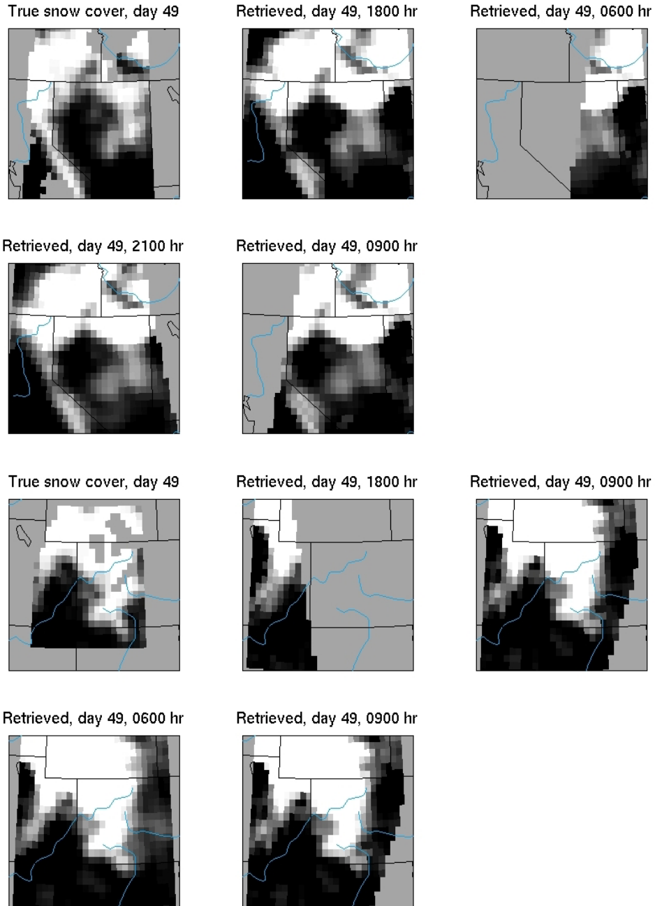
Figure 5-3: True (day 49) and retrieved (day 49) snow cover maps. Top: California-Nevada. Bottom: Colorado-Utah
